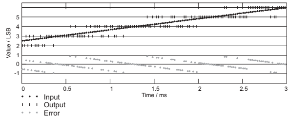
Figure 115. Quantization of a ramp with RPDF dither.
