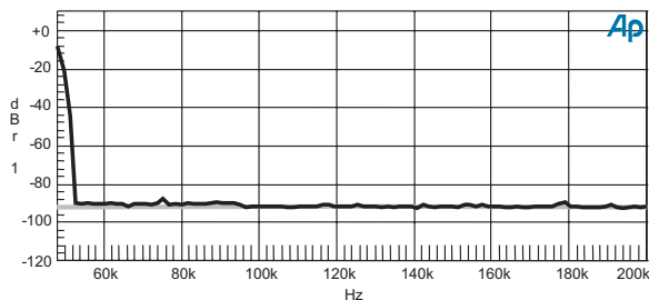
Figure 28. Anti-alias filter stopband attenuation.
