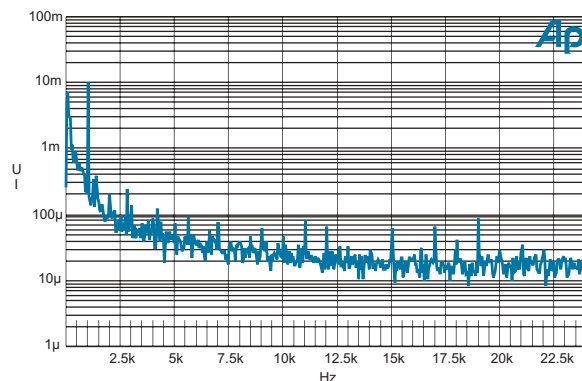
Figure 5. FFT spectrum analysis of jitter signal.
