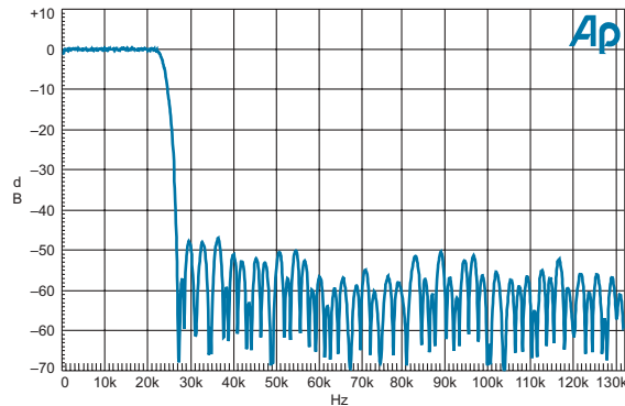
Figure 58. Anti-image filter.
