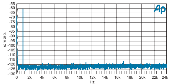
Figure 39. FFT of signal-to-noise test output, linear axis.
