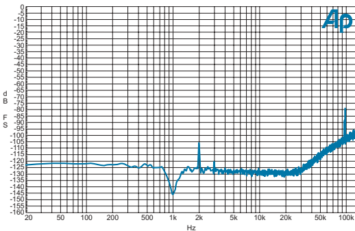
Figure 91. FFT of THD+N test notch filter output, logarithmic scale.
