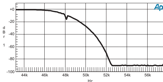
Figure 29. Anti-alias filter transition region.
