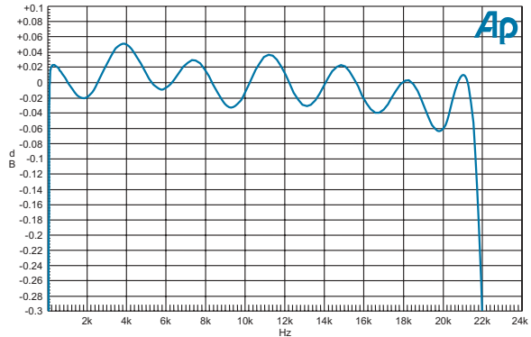
Figure 66. DAC “B” passband, linear frequency plot.
