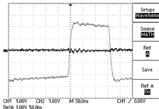
Figure 136. Oscilloscope view of sum (black) and difference (gray) of balanced interface signal legs.
