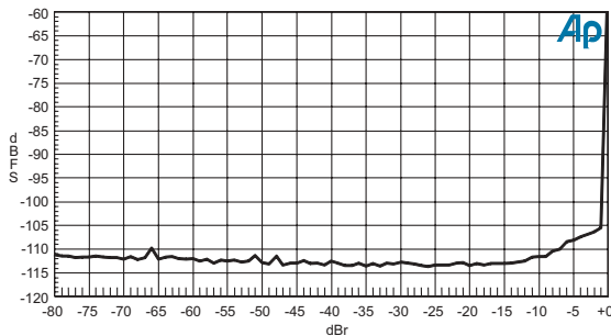
Figure 43. THD+N by level for a 997 kHz tone. The plot shows THD+N (dB FS) on the y-axis (ranging from -120 to -60) versus level (dB) on the x-axis (ranging from -80 to +0). The curve shows a relatively flat line around -110 dB FS until about -10 dB, where it begins to rise sharply towards -60 dB FS at 0 dB. A blue 'Ap' logo is in the top right corner.
