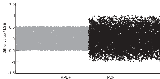
Figure 113. Rectangular and Triangular dither.
