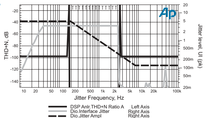
Figure 151. Device THD+N plotted against jitter.
